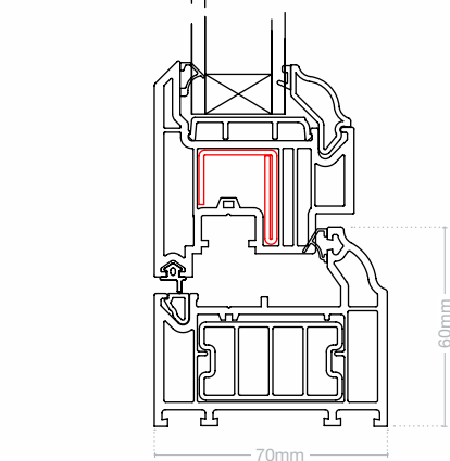
HORIZONTAL CROSS SECTION
