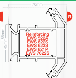
Intermediate transom T EWS 7022
