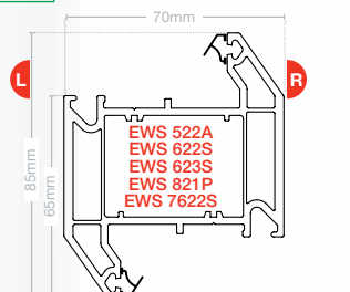
Intermediate transom Z EWS 7023
